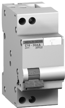
Fig. H26 : Domestic-type circuit-breaker as above (Fig. H25) with incorporated protection against electric shocks
