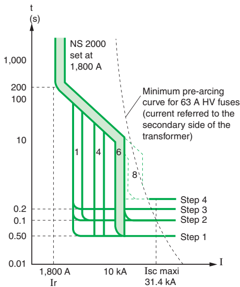
Fig. H58 : Curves of MV fuses and LV circuit-breaker
