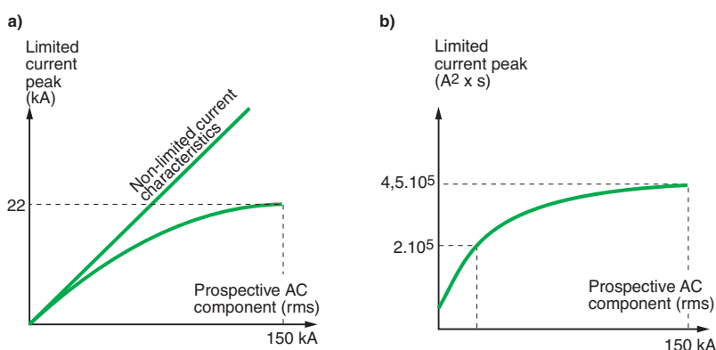
Fig. H39 : Performance curves of a typical LV current-limiting circuit-breaker
