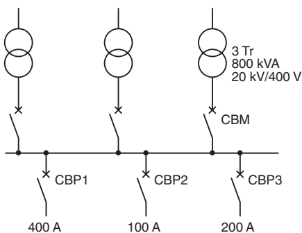
Fig. H47 : Transformers in parallel
